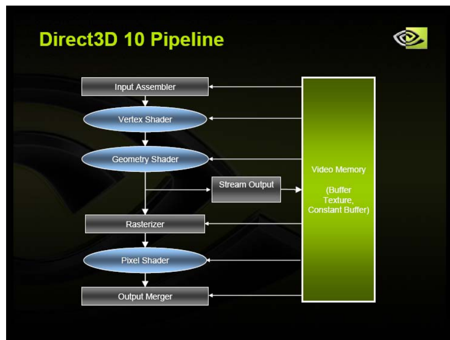
Figure 6 The DirectX 10 pipeline adds the geometry shader and stream output, allowing for iterative calculations on the GPU with no CPU intervention.
