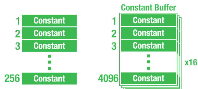
Figure 8 In DirectX 9 (left), only 256 registers are available. DirectX 10 (right) offers sixteen constant buffers of 4096 constants each.
