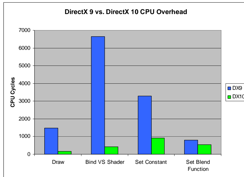
Figure 3. DirectX 9 vs. DirectX 10 CPU Overhead
